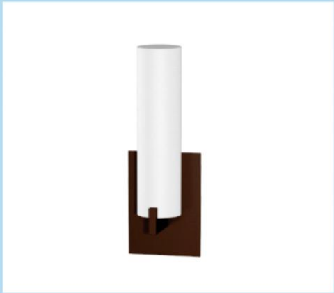
Model No: B600604 Dimensions: 14" H x 5" W x 4.5" D Finish: Bronze Base/Wall Plate: 8" H x 5" W Socket: 1xGU24 Shade Material: Frosted acrylic Shade Style: Straight round Shade Dimensions: 3" Dia. x 11.5" H Wattage: 5~18W LED
